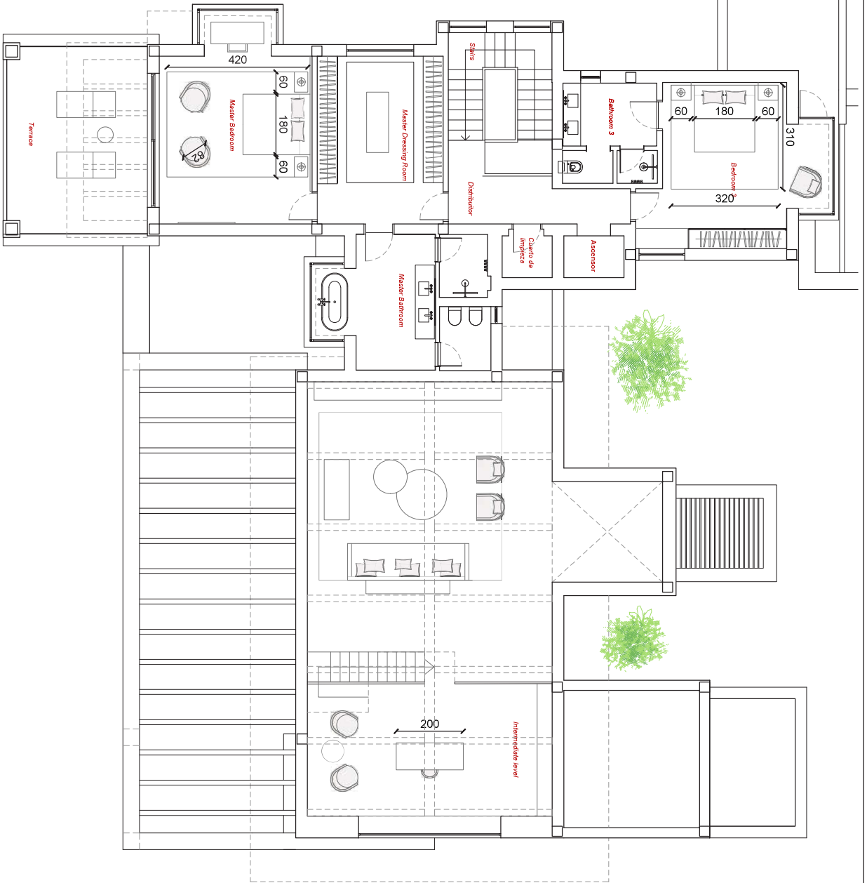
A02. FLOOR PLAN LAYOUT. FIRST FLOOR
